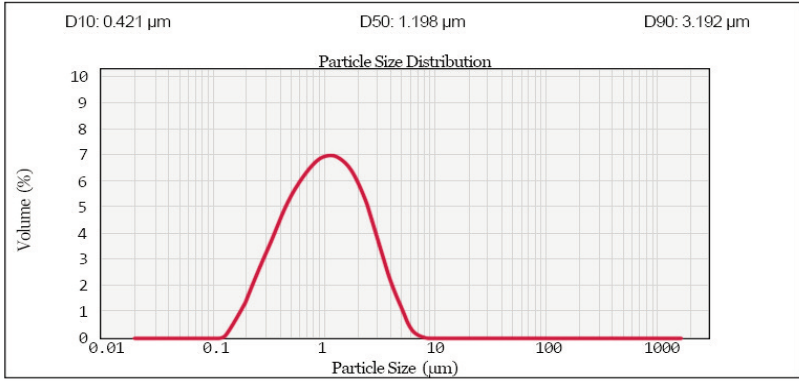
Ceroxid HD W1015 PSD laser particle size distribution analyzer
